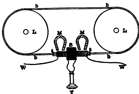
FIG. 48.—Magnetic Receiver.
